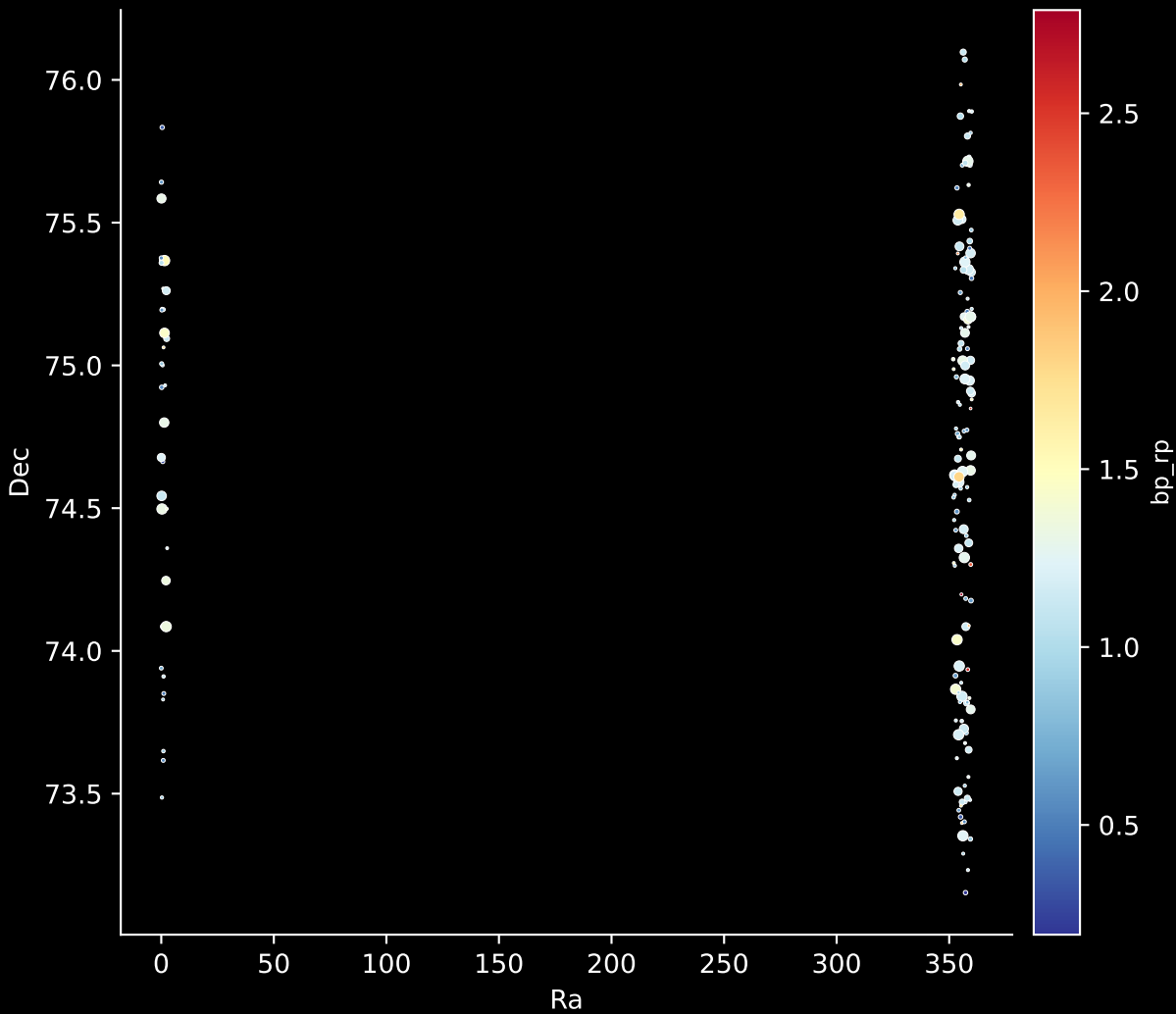
APOGEE DR17 Field: [CVZTILE_106+33_btx] Stars: 173
