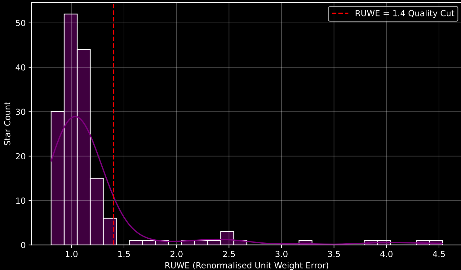
GAPOGEE DR17 Field [CVZTILE_106+33_btx] RUWE Distribution (n= 162)
