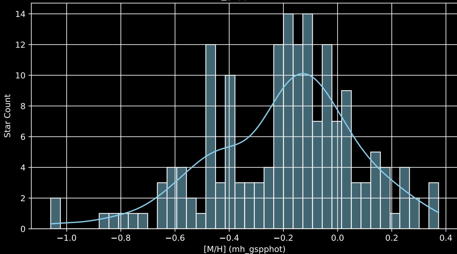
APOGEE DR17 Field: [CVZTILE_106+33_btx [M/H] (mh_gspphot) (n= 171)
