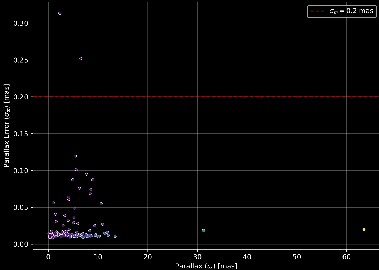
APOGEE DR17 Field: [CVZTILE_106+33_btx] Parallax Quality (n= 173)
