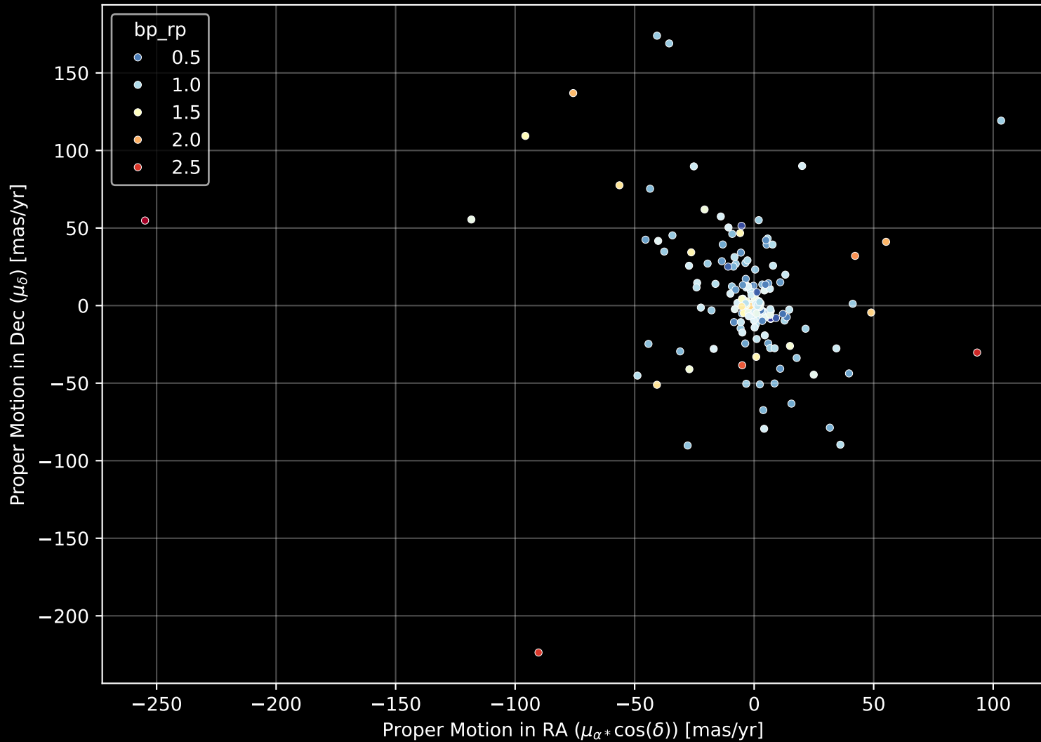
APOGEE DR17 Field: [CVZTILE_106+33_btx] Proper Motion Diagram (n= 173)
