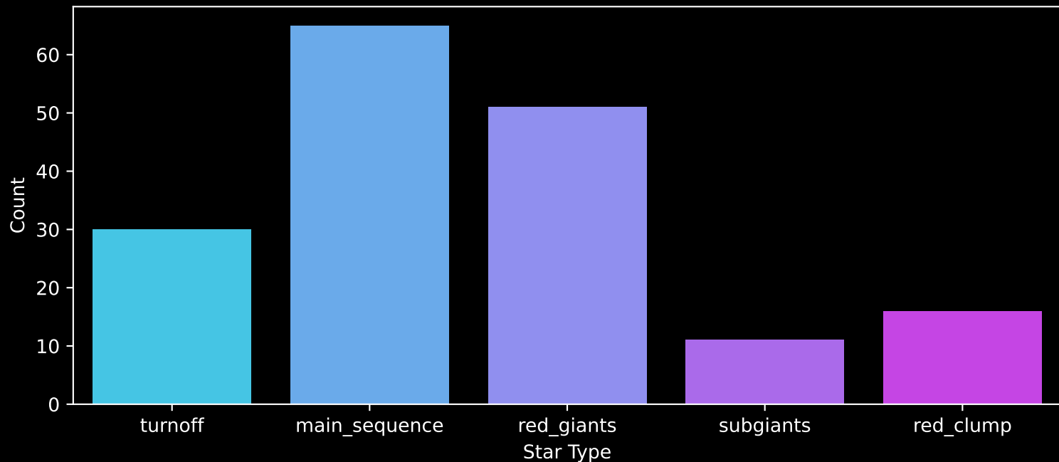
APOGEE DR17 Field: [CVZTILE_106+33_btx] Count plot of Star Type
